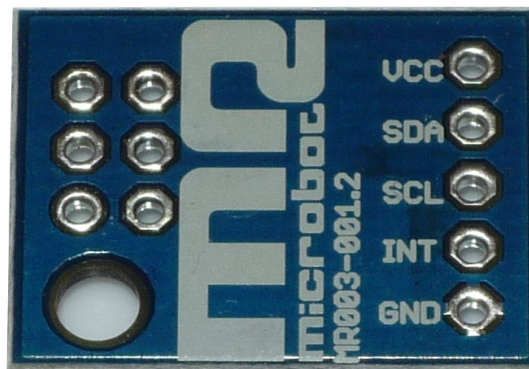
Fig. 2 - Signals
