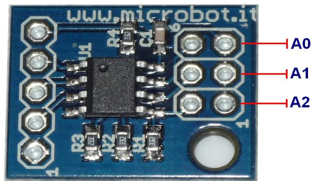
Fig. 1 - Slave address jumpers
